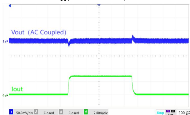
动态负载 I_{OUT}=0.1\text{A}\sim 3\text{A}\sim 0.1\text{A} , 6\text{A}/\mu\text{s}
