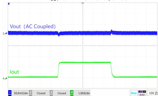
动态负载 I_{OUT}=0.1\text{A}\sim 1.5\text{A}\sim 0.1\text{A} , 6\text{A}/\mu\text{s}
