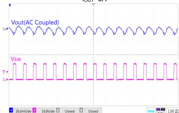
V_{OUT} 纹波 I_{OUT}=0\text{A}
