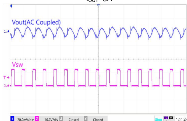
V_{OUT} 纹波 I_{OUT}=3\text{A}
