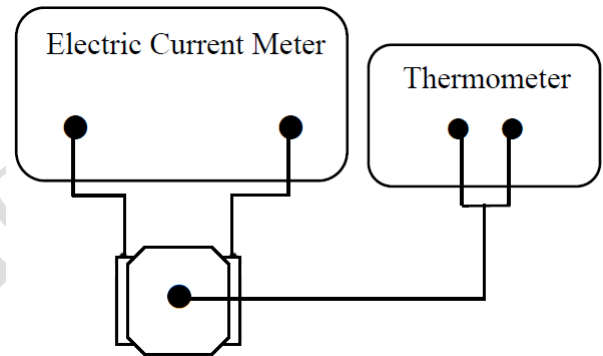
Irms test schematic diagram
