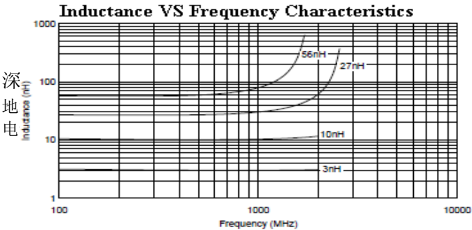
电性特征曲线图 Typical Electrical Characteristics
